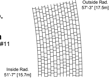
10 ° Section
