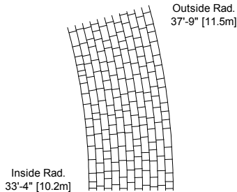
15 ° Section
