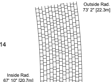
8 ° Section
